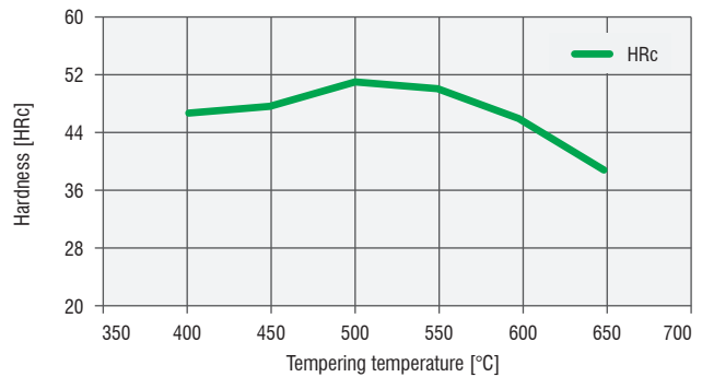
Tempering curve
