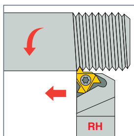
Right-Hand Thread
