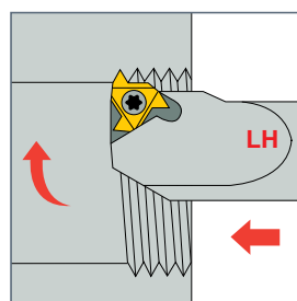
Left-Hand Thread
